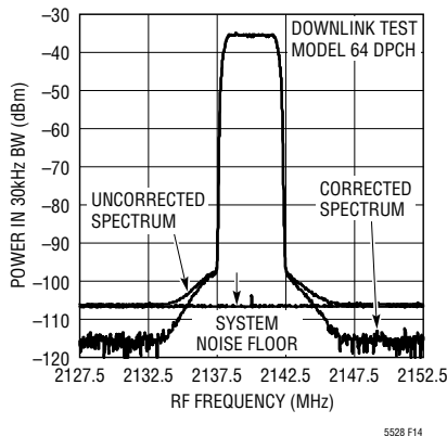
Figure 14: 1-Channel W-CDMA Spectrum
