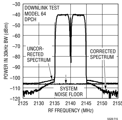
Figure 15: 2-Channel W-CDMA Spectrum
