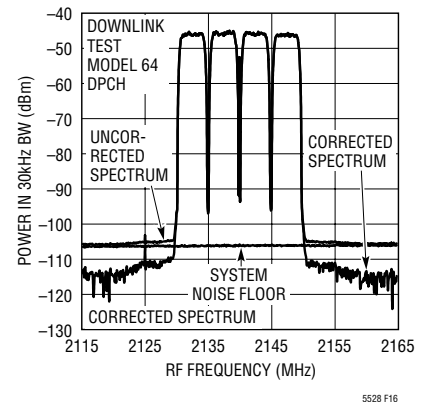
Figure 16: 4-Channel W-CDMA Spectrum
