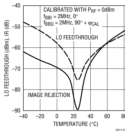
LO Feedthrough and Image Rejection vs Temperature After Calibration at 25^\circ C
