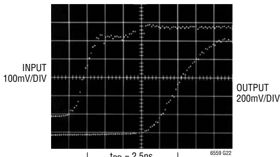
Propagation Delay
