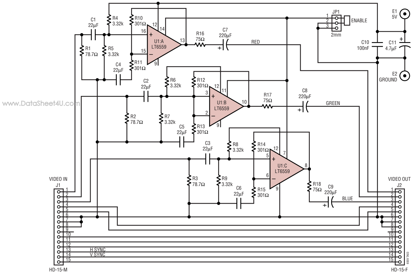
DC1063A Demo Circuit Schematic
