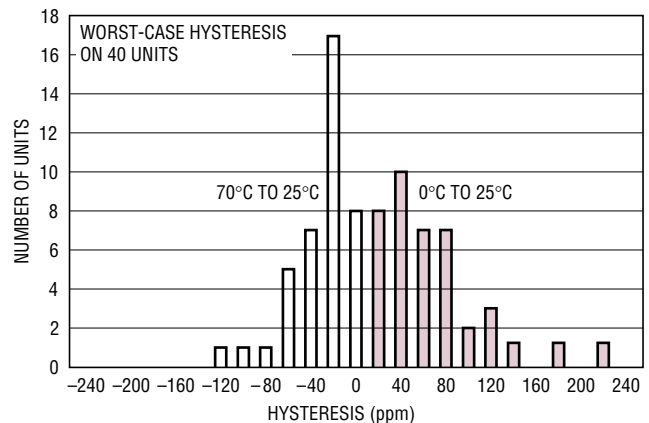
Figure 6. 0^\circ C to 70^\circ C Hysteresis
