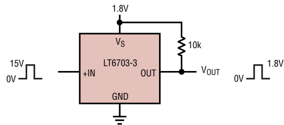
Level Translator High Voltage to Low Voltage
