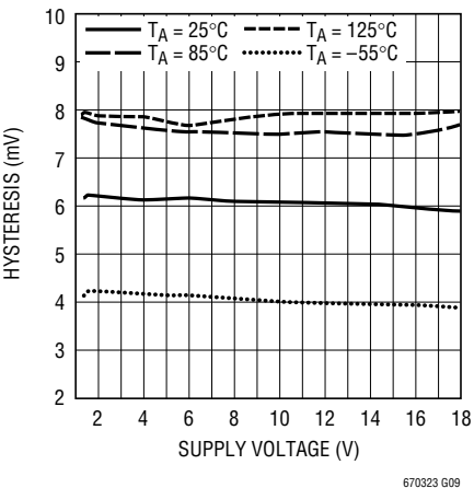
Hysteresis vs Supply Voltage
