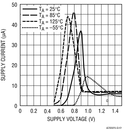
Start-Up Supply Current
