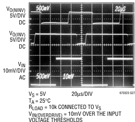
Noninverting and Inverting Comparator Propagation Delay
