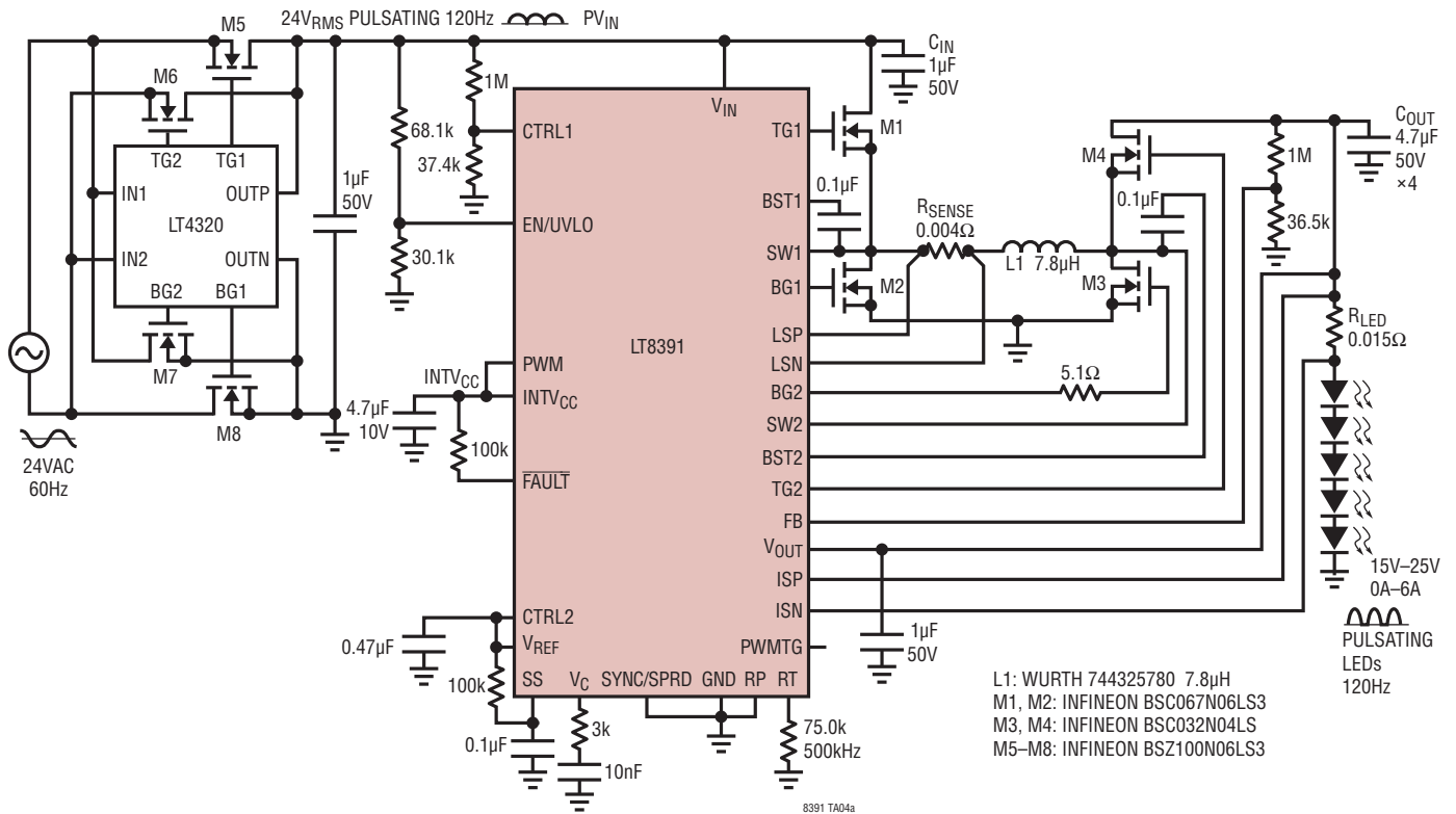
93% Efficient 84W Buck-Boost LED Driver from 24VAC
