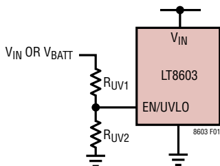
Figure 1. UVLO Divider
