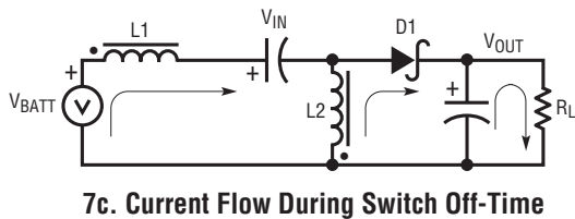
Figures 7. SEPIC Topology and Current Flow
