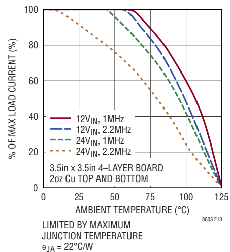
Figure 13. Thermal Derating, E- and I-Grade
