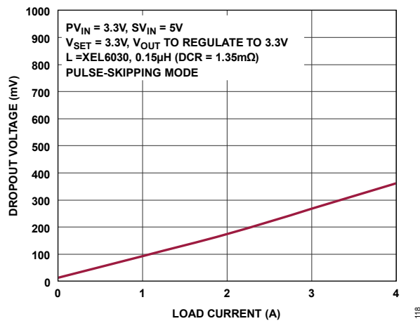
Figure 22. PV_{IN} Dropout Voltage
