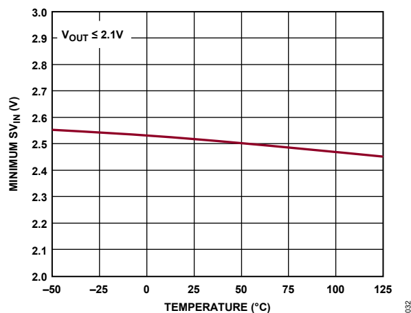
Figure 26. Minimum SV_{IN}
