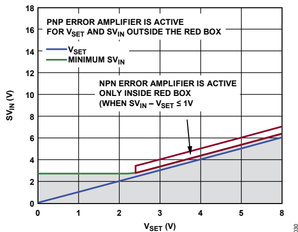
Figure 24. Minimum SV_{IN} as a Function of V_{SET}
