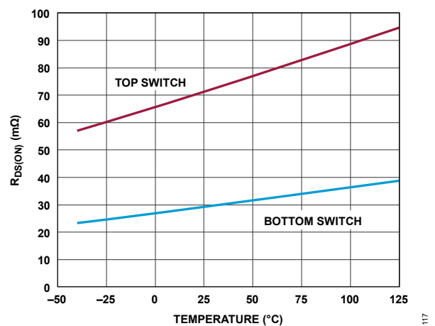
Figure 21. Switch R_{DS(ON)} vs Temperature
