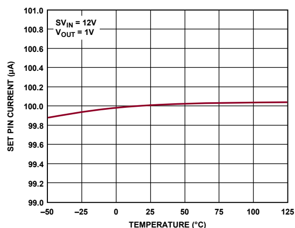
Figure 15. SET Pin Current
