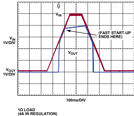
Figure 45. Start-Up Dropout Performance
