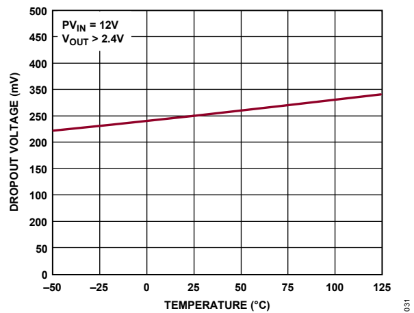
Figure 25. SV_{IN} Dropout Voltage
