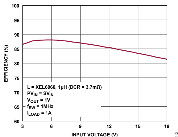
Figure 14. Efficiency vs V IN
