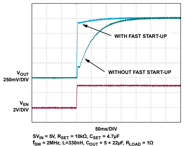
Figure 33. Start-Up Time with and without Fast Start-Up Circuitry for Large CSET
