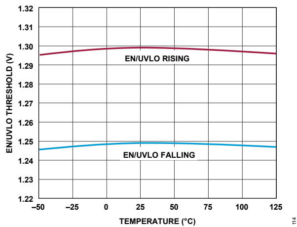
Figure 18. EN/UVLO Pin Thresholds
