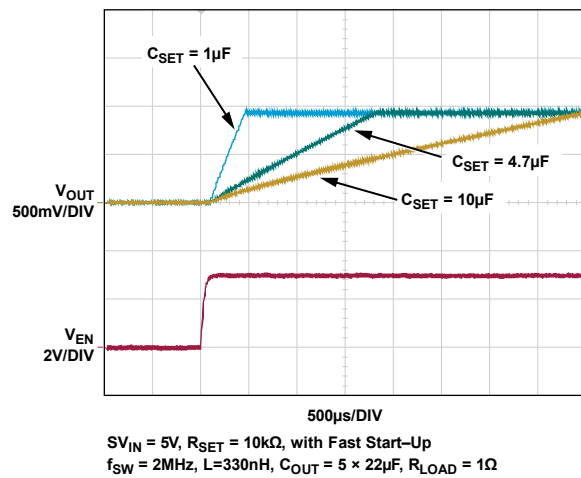
Figure 34. Soft-Start Waveforms
