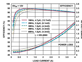
Figure 2. 12V IN to 5V OUT Efficiency
