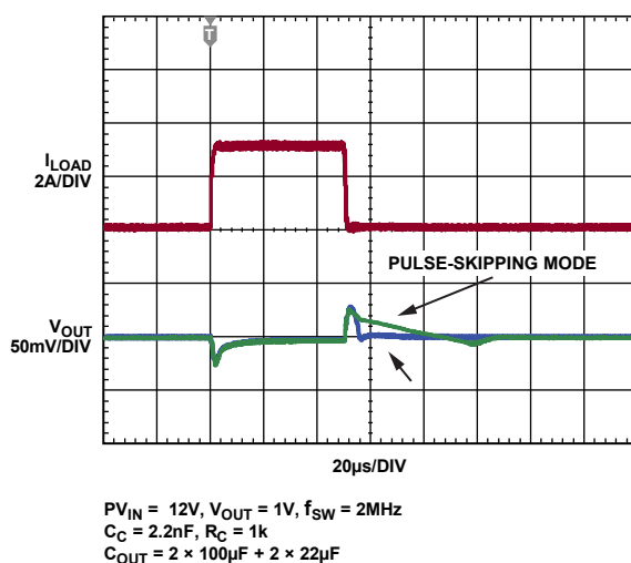
Figure 55. Load Step Transient Response with and without Forced Continuous Mode
