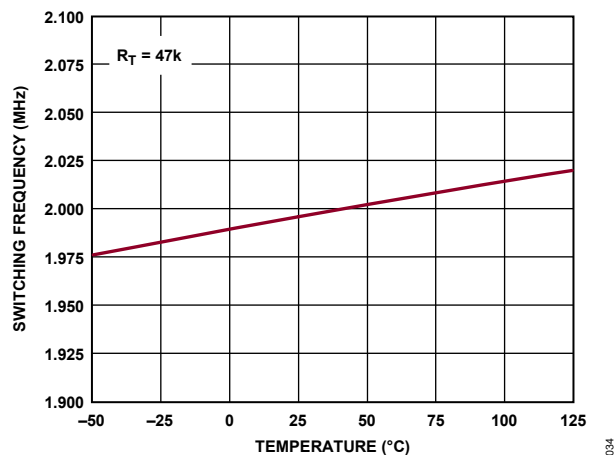
Figure 28. Switching Frequency
