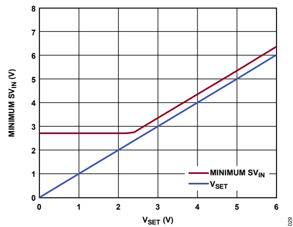
Figure 23. Minimum SV_{IN} as a Function of V_{SET}
