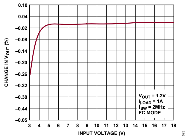
Figure 17. Line Regulation
