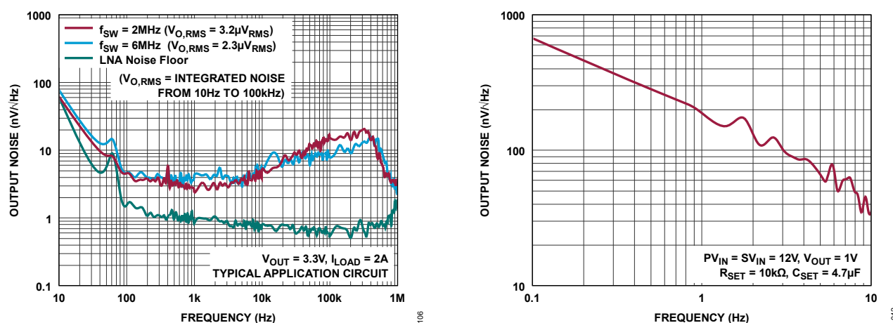
Figure 51. Noise Spectral Density
