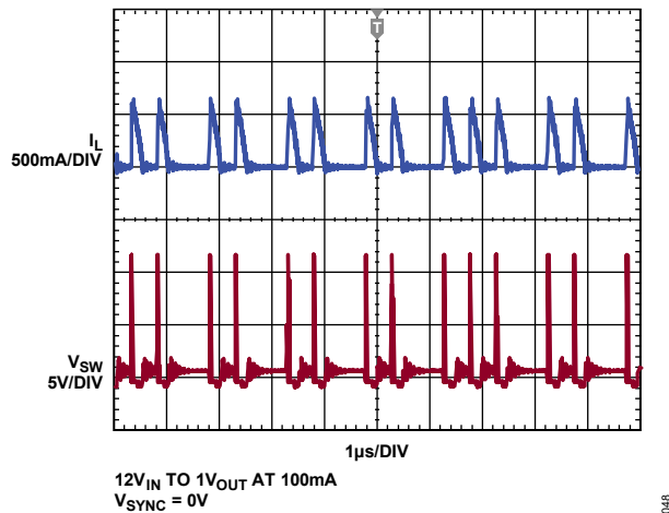
Figure 42. Switching Waveforms, Pulse-Skipping Operation
