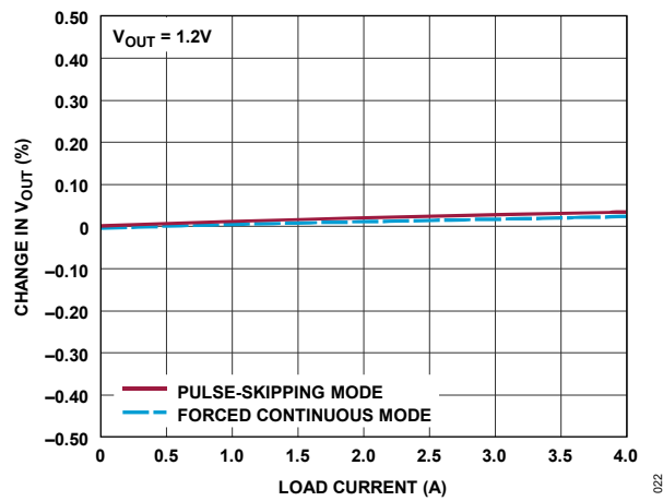
Figure 16. Load Regulation
