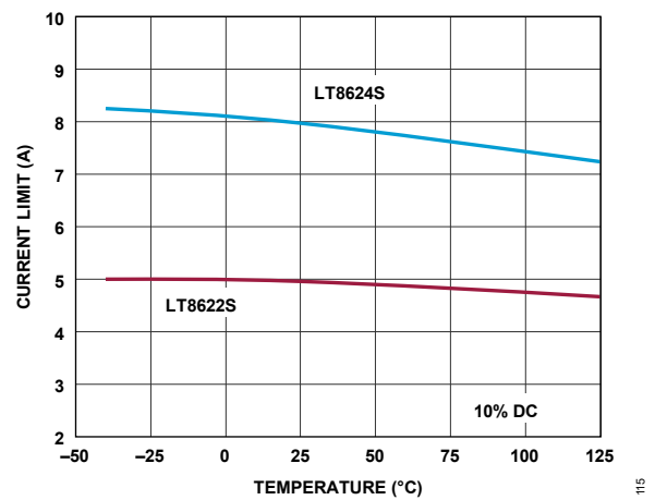
Figure 19. Top MOSFET Current Limit
