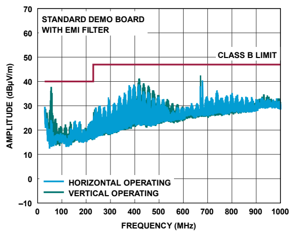
Figure 49. LT8624S Radiated EMI Performance (CISPR32 Radiated Emission Test with Class B Limits)
