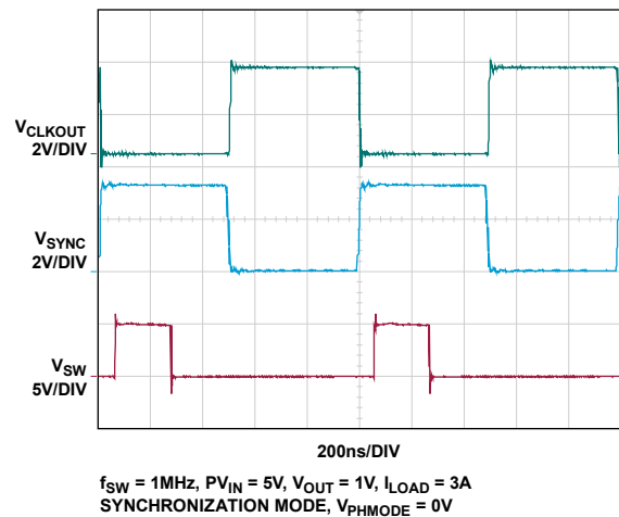
Figure 43. CLKOUT Waveforms
