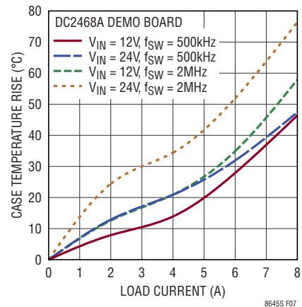
Figure 7. Case Temperature Rise
