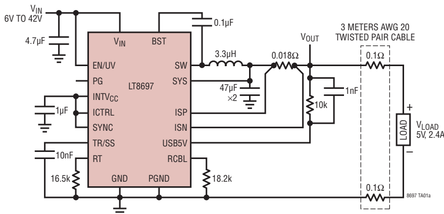
2MHz 5V Step-Down Converter with Cable Drop Compensation
