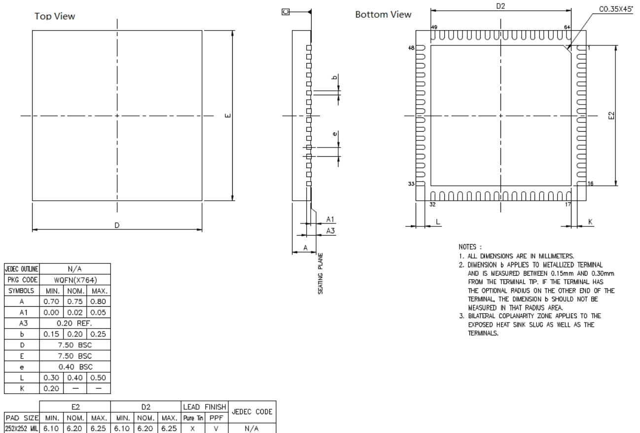
Fig6.2 LT8912B QFN64 7.5mmx7.5mm Package
