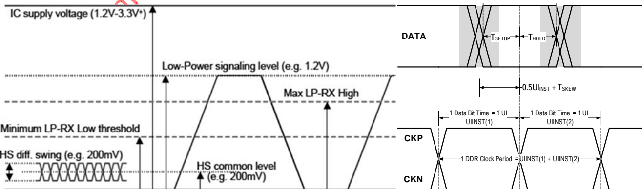
Fig 5.2.1 MIPI Rx D-PHY Electrical Parameter and Timing Definitions: (Left) Line Levels; (Right) DDR Clock and Data-to-Clock Timing
