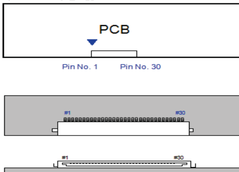
Fig. Connector diagram
