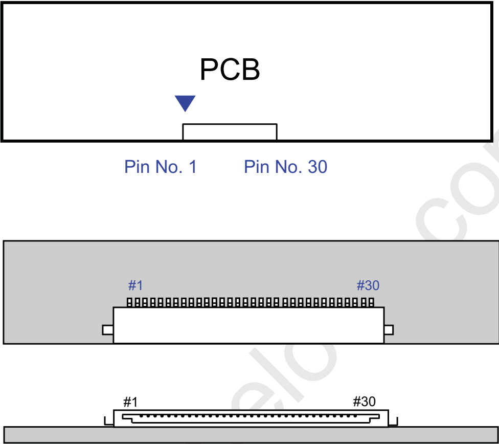
Fig. Connector diagram
