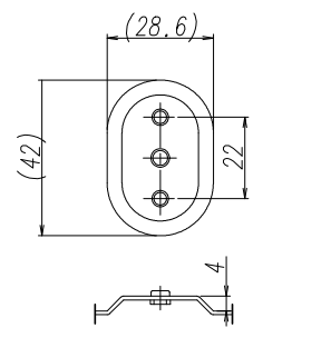
DETAIL "A" (2PARTS)
