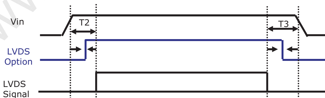
LVDS Option Sequence
