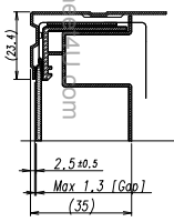
SECT;A-A(2/1)
