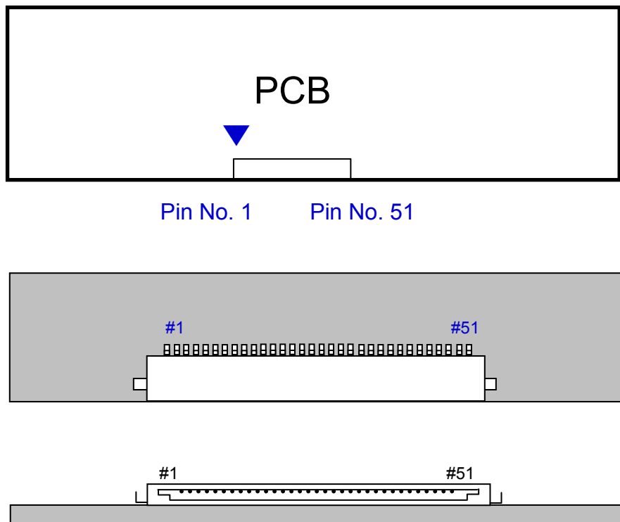
Fig. Connector diagram
