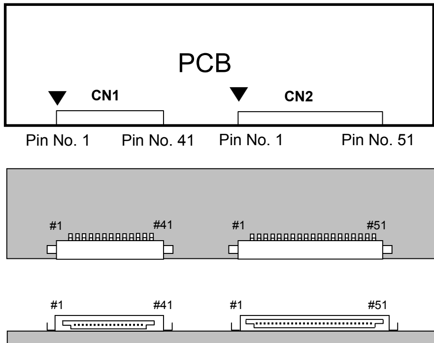
Fig. Connector diagram
