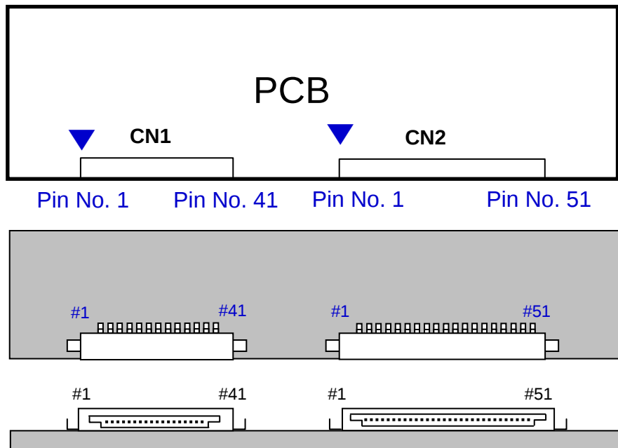
Fig. Connector diagram
