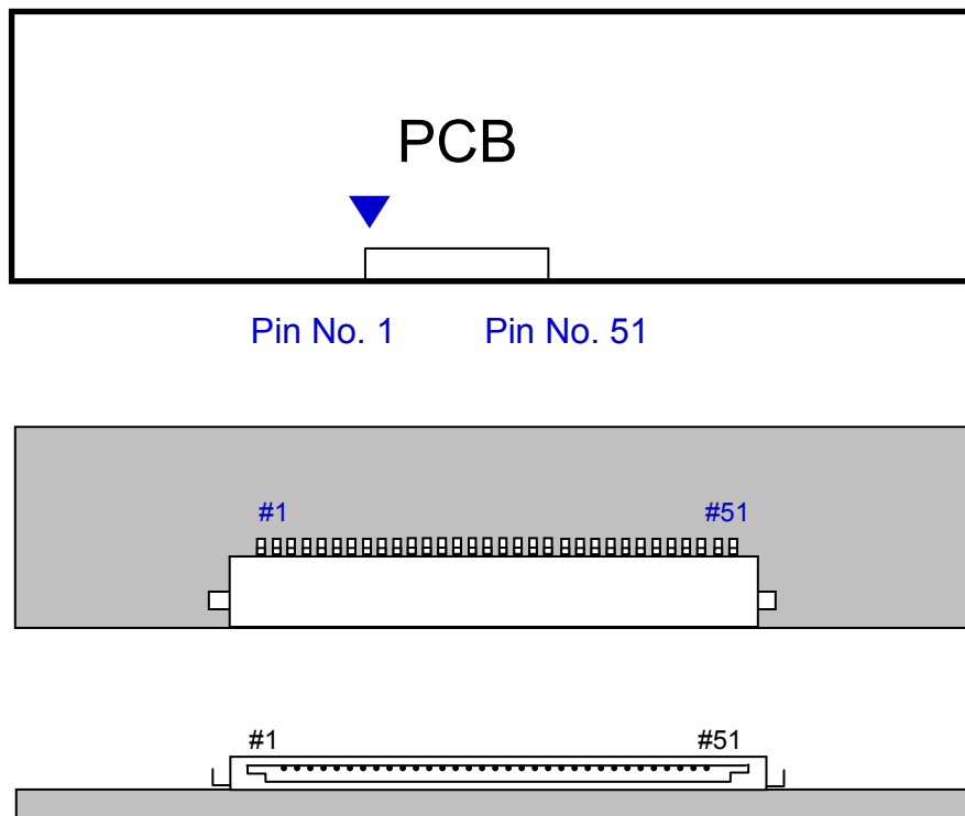
Fig. Connector diagram
