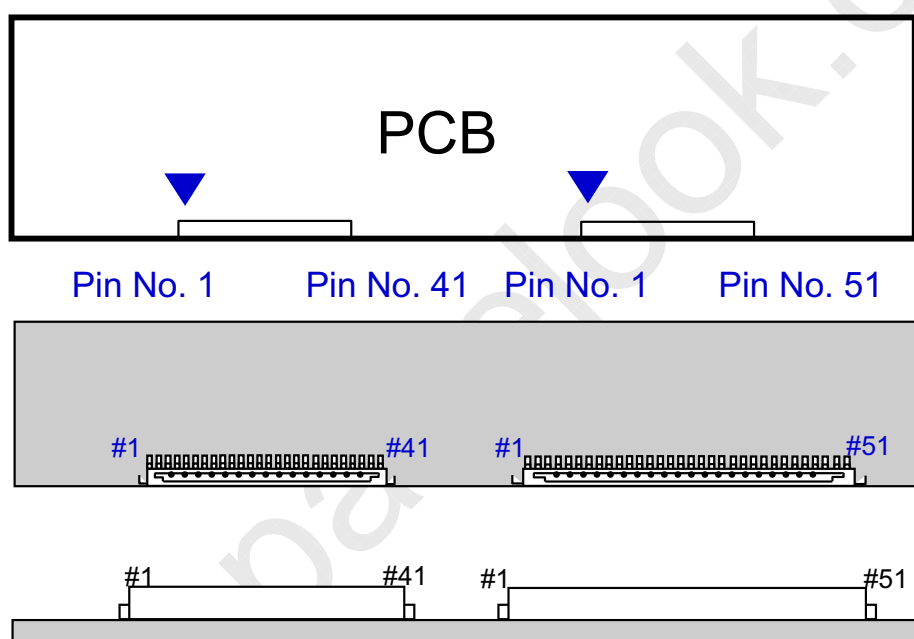
Fig. Connector diagram
