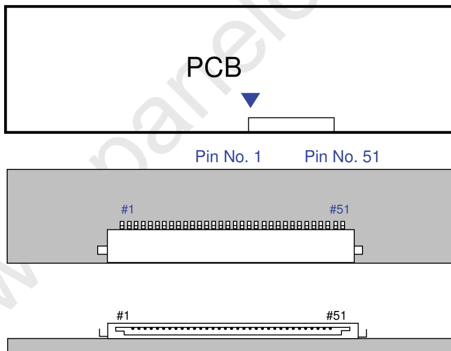
Fig. Connector diagram
