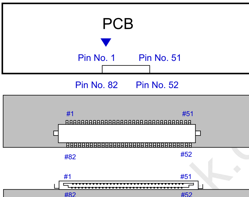
Fig. Connector diagram
