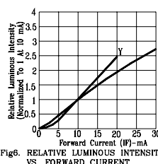
Fig6. RELATIVE LUMINOUS INTENSITY VS. FORWARD CURRENT
