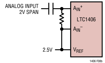
Figure 8b. AC Coupled
