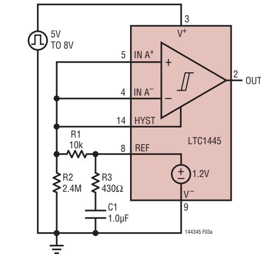
Figure 3a. V + Glitching Test Circuit
