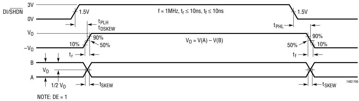
Figure 6. Driver Propagation Delays
