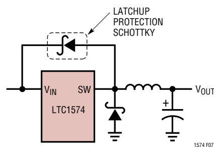
Figure 7. Preventing Absolute Maximum Ratings from Being Exceeded
