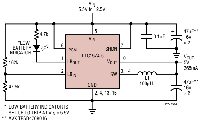
Low Dropout 5V Step-Down Regulator with Low-Battery Detection
