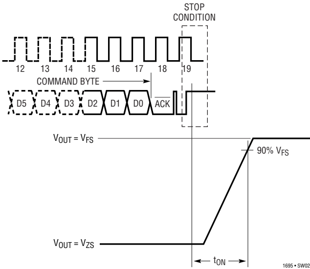
Output Switch On Time Measurement Code = 63, I_{LOAD} = 1mA, C_{LOAD} = 4.7\mu F f_{SMBus} = 100kHz
