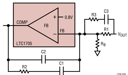
Figure 3. "Type 3" Feedback Loop (I/O Channel)
