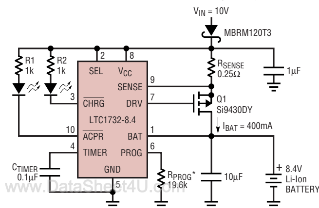
400mA 2-Cell 8.4V Li-Ion Battery Charger
