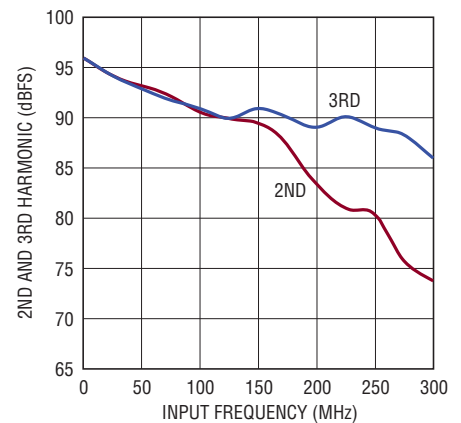
2nd, 3rd Harmonic vs Input Frequency, -1dBFS, 20MSPS, 1V Range
