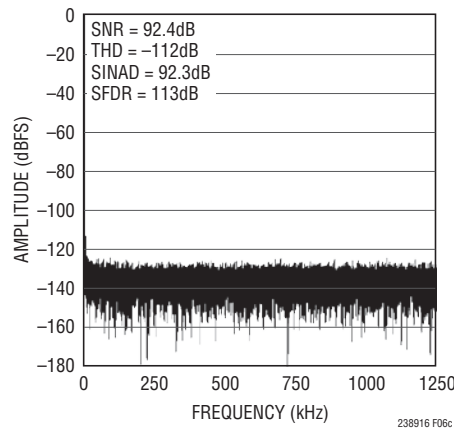
Figure 6c. 32k Point FFT f_{\text{SAMPL}} = 2.5\text{Msps} , f_{\text{IN}} = 2\text{kHz} , for Circuit Shown in Figure 6a; Driven with Unipolar Inputs
