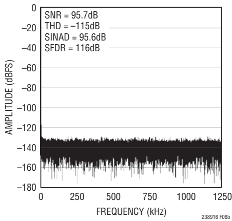
Figure 6b. 32k Point FFT f_{\text{SAMPL}} = 2.5\text{Msps} , f_{\text{IN}} = 2\text{kHz} , for Circuit Shown in Figure 6a; Driven with Fully Differential Inputs
