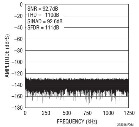
Figure 6d. 32k Point FFT f_{\text{SAMPL}} = 2.5\text{Msps} , f_{\text{IN}} = 2\text{kHz} , for Circuit Shown in Figure 6a; Driven with Bipolar Inputs
