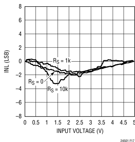
Figure 17. Measured INL vs V_{IN} , C_{IN} = 0 , V_{CC} = 5V , T_A = 25^\circ C
