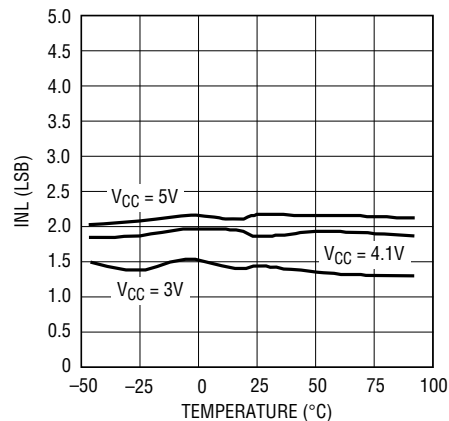
Maximum INL vs Temperature
