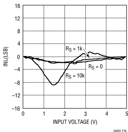
Figure 16. Measured INL vs Input Voltage, C_{IN} = 0.1\mu F, V_{CC} = 5V , T_A = 25^\circ C
