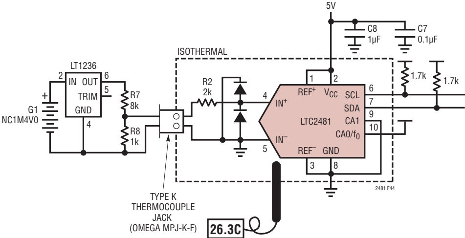
Figure 44. Calibration Setup
