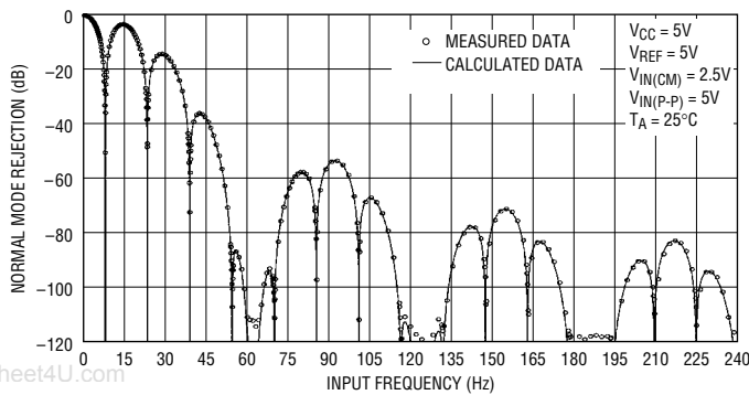
Figure 30. Input Normal Mode Rejection vs Input Frequency with Input Perturbation of 100% Full Scale (60Hz Notch f_{EOSC} = 307.2\text{kHz} )
