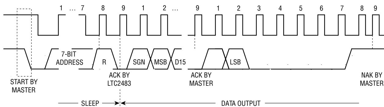
Figure 3. Timing Diagram for Reading from the LTC2483
