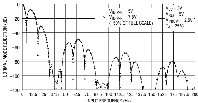
Figure 34. Measured Input Normal Mode Rejection vs Input Frequency with Input Perturbation of 150% Full Scale (50Hz Notch f_{EOSC} = 256\text{kHz} )
