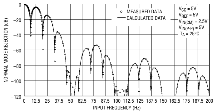
Figure 31. Input Normal Mode Rejection vs Input Frequency with Input Perturbation of 100% Full Scale (50Hz Notch f_{EOSC} = 256\text{kHz} )
