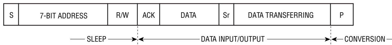
Figure 4. The LTC2483 Conversion Sequence
