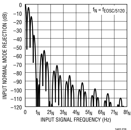
Figure 28. Input Normal Mode Rejection at DC
