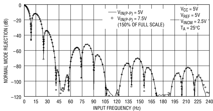
Figure 33. Measured Input Normal Mode Rejection vs Input Frequency with Input Perturbation of 150% Full Scale (60Hz Notch f_{EOSC} = 307.2\text{kHz} )
