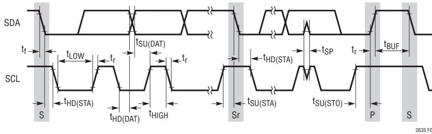
Figure 1. I 2 C Timing
