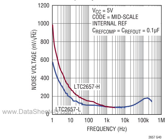
Noise Voltage Density vs Frequency
