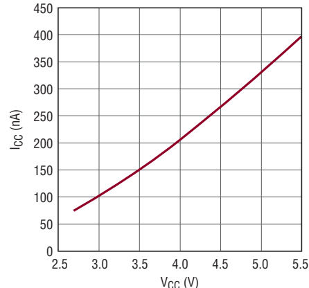
I_{CC} Shutdown vs V_{CC}
