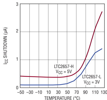
I_{CC} Shutdown vs Temperature
