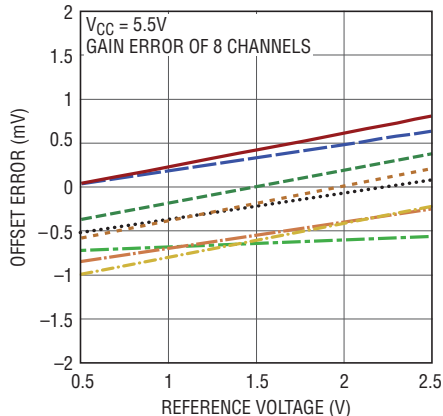
Offset Error vs Reference Input
