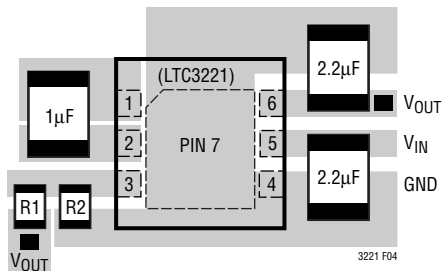
Figure 4. Recommended Layout
