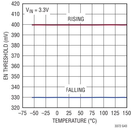
Precise Enable Threshold vs Temperature
