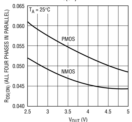
Effective R_{DS(ON)}
