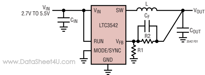
Figure 1. LTC3542 General Schematic
