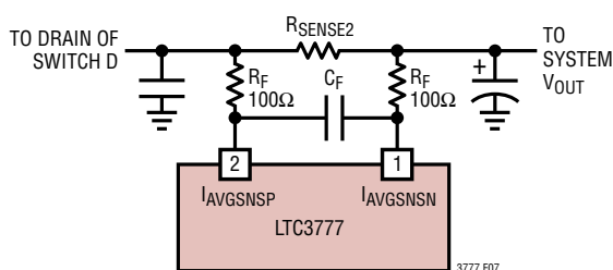
Figure 7. Programming Output Current Limit
