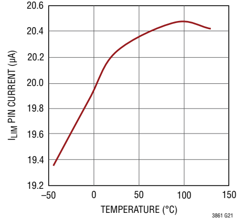
I_{LIM} Pin Current vs Temperature
