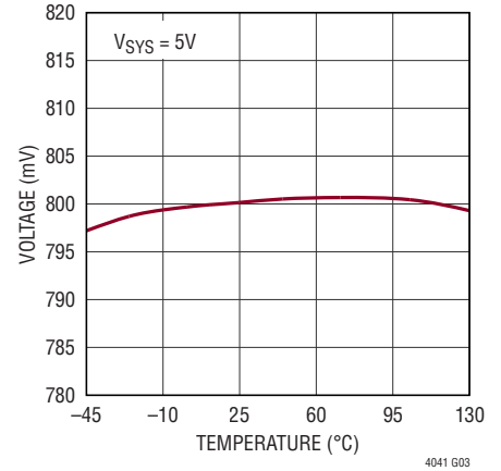
V_{CAPFB} vs Temperature
