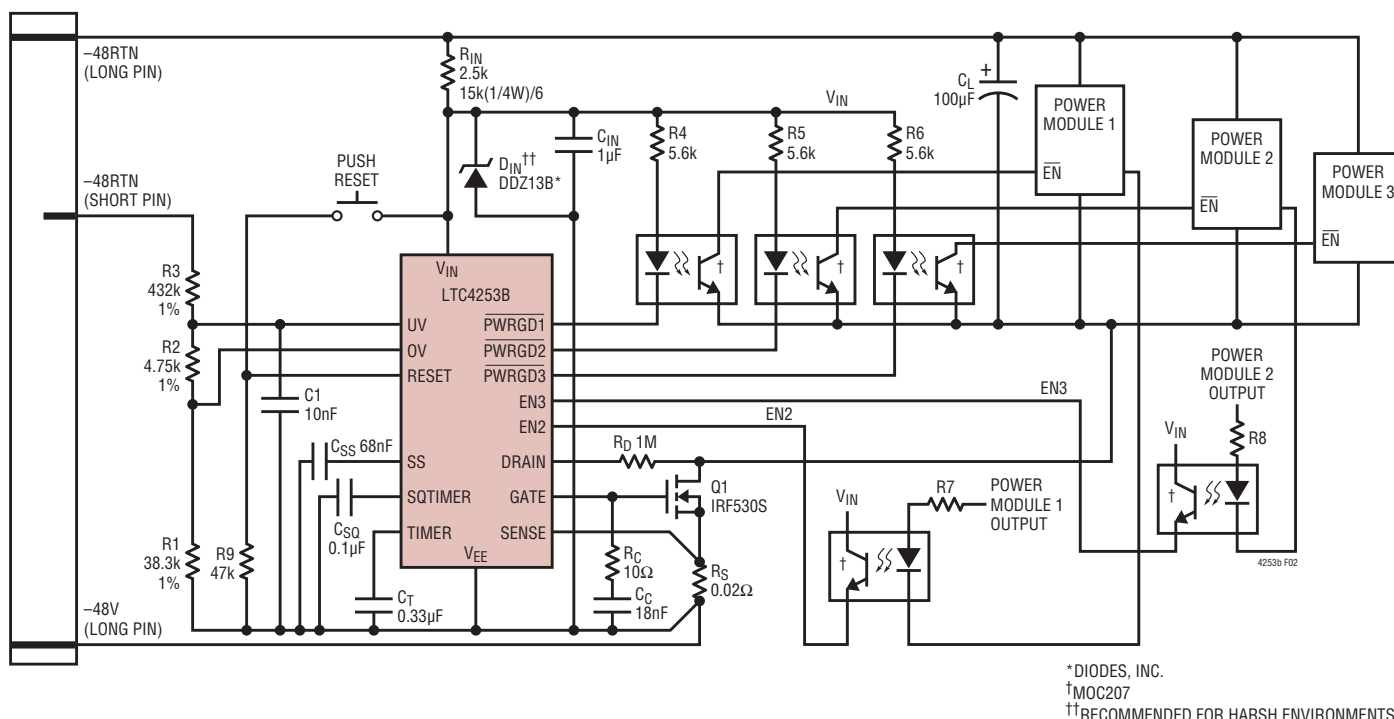
Figure 2. -48V/2.5A Application with a Wider Operating Range
