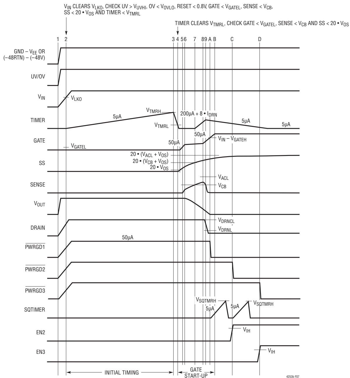
Figure 7. System Power-Up Timing (All Waveforms Are Referenced to V_{EE} )
