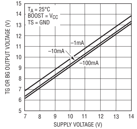
Output High Voltage ( V_{\text{OH}} ) vs Supply Voltage
