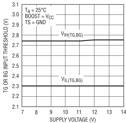
Input Thresholds ( T_{\text{INP}} , \text{BINP} ) vs Supply Voltage
