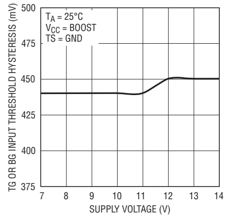
Input Thresholds ( T_{\text{INP}} , \text{BINP} ) Hysteresis vs Voltage
