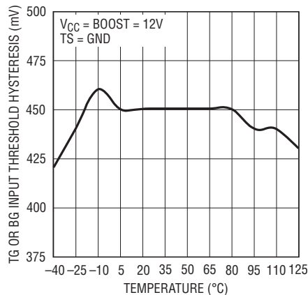
Input Thresholds ( T_{\text{INP}} , \text{BINP} ) Hysteresis vs Temperature
