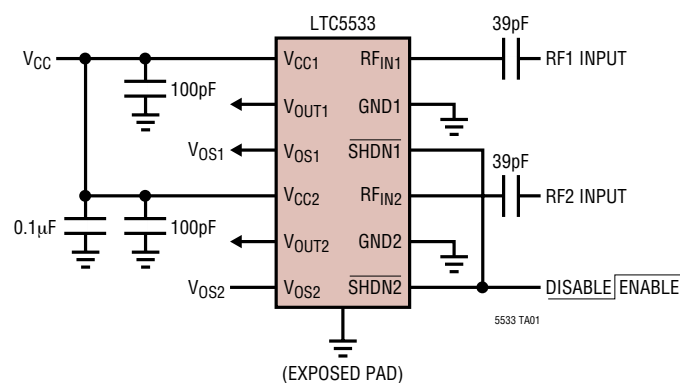
300MHz to 11GHz RF Power Detectors
