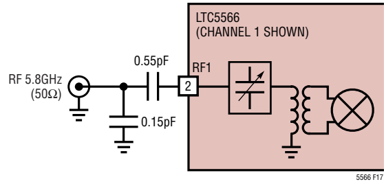
Figure 17. 5.8GHz Input Matching
