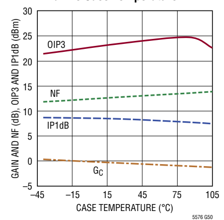
Conversion Gain, OIP3, NF and IP1dB vs Case Temperature
