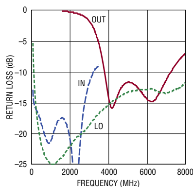
IN, OUT and LO Return Loss vs Frequency
