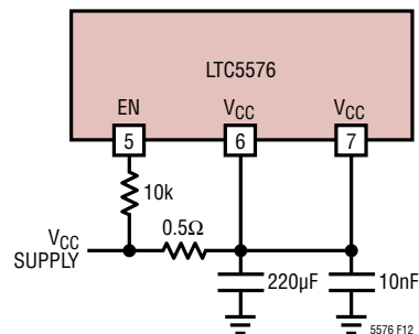
Figure 12. Suggested Configuration for Simultaneous V CC and EN Switching
