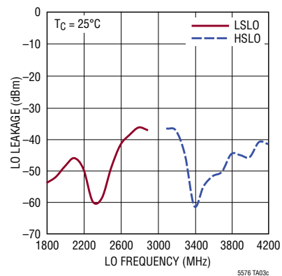
LO-OUT Leakage vs LO Frequency
